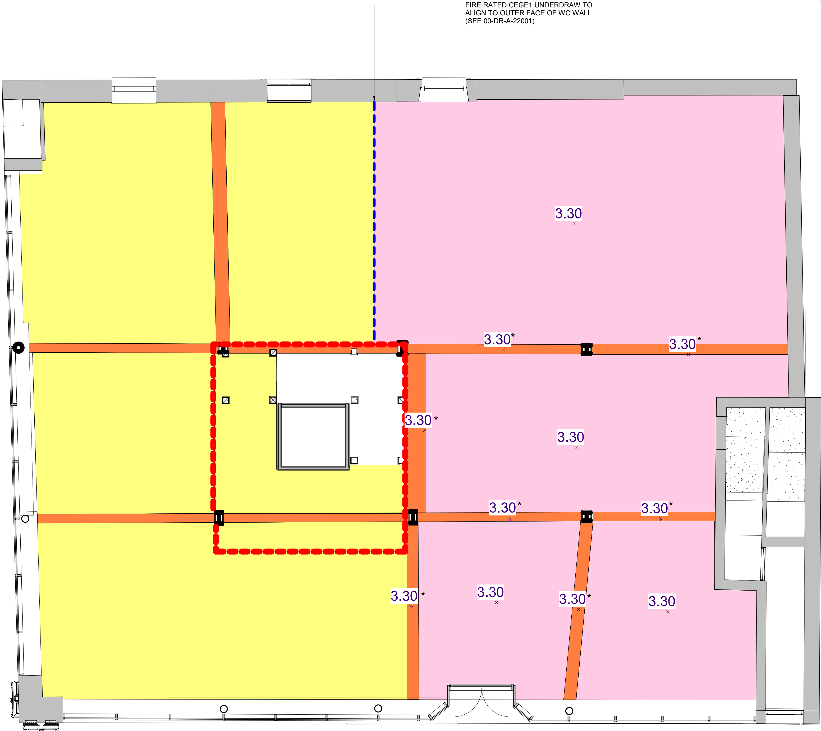
LEVEL 00 CEILING LININGS SCALE: 1 : 50
