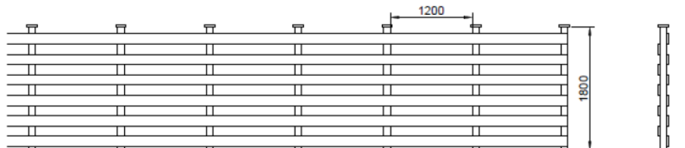
1800mm hit and miss privacy fence (example)
