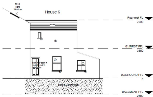
Elevation 6 (house 6 side elevation) 1 : 100
