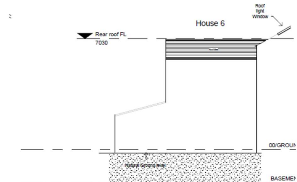
Elevation 6a (house 6 side elevation) 1 : 100
