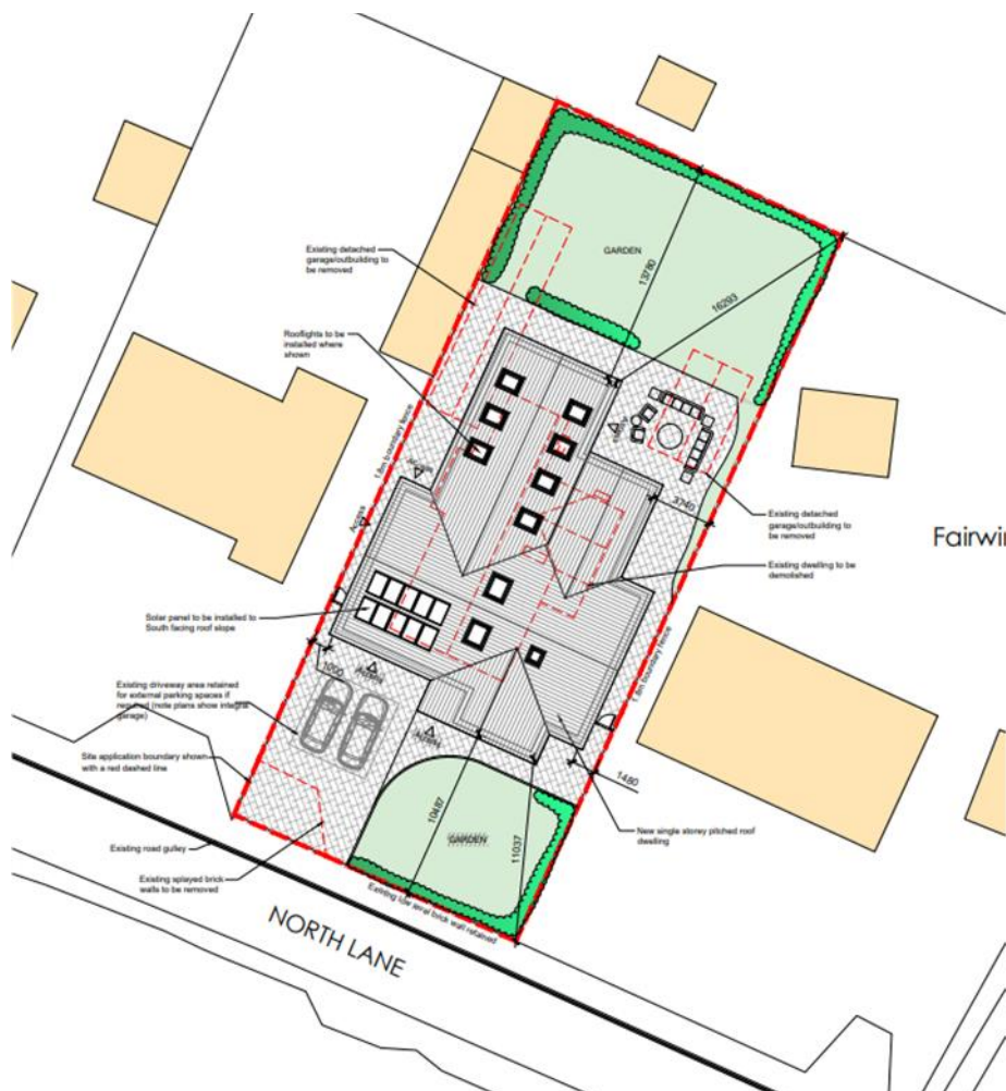
(Fig.14 – Extract of drawing 24-36-P-01 showing the proposed site layout)
