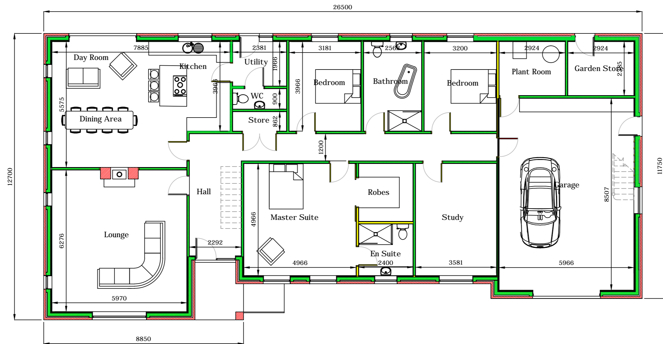
Floor Plan
