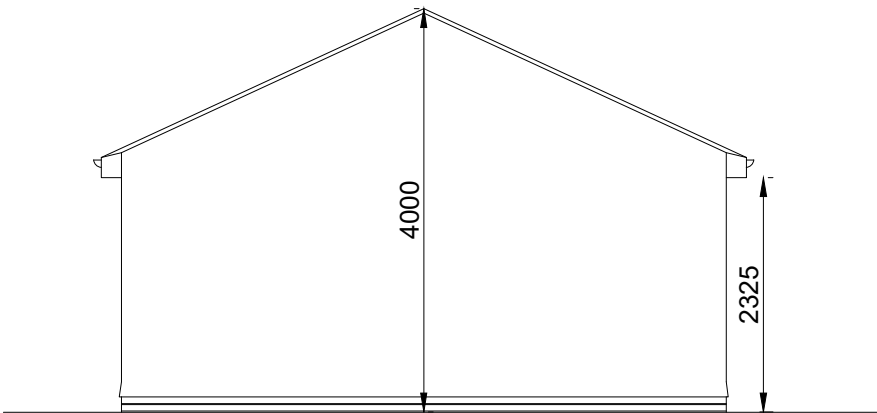
Rear Elevation
