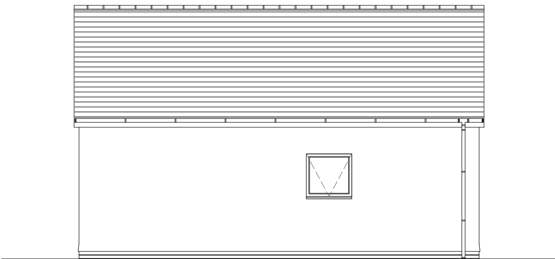
Side Elevation
