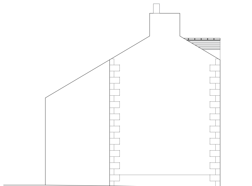
Side Elevation
