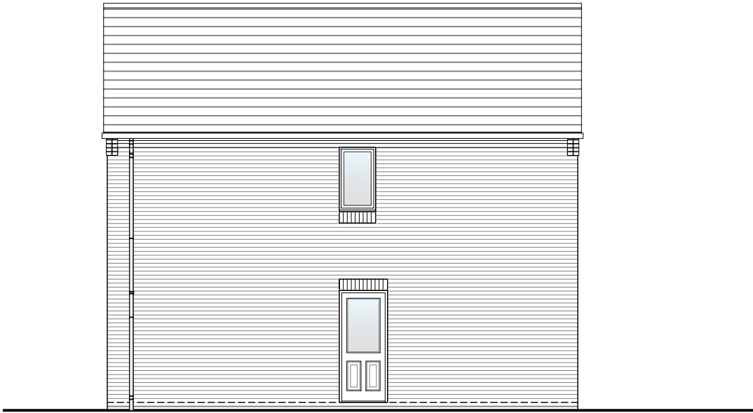
Rear Elevation
