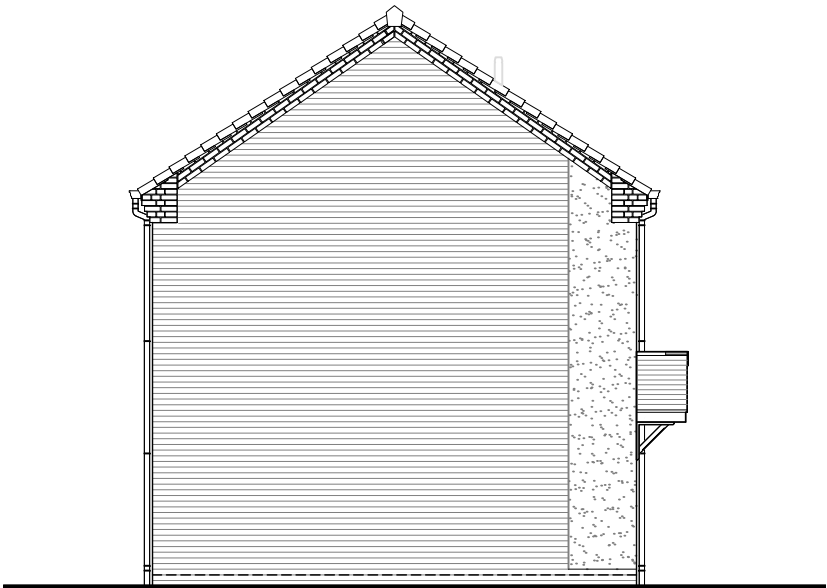
Left Elevation
