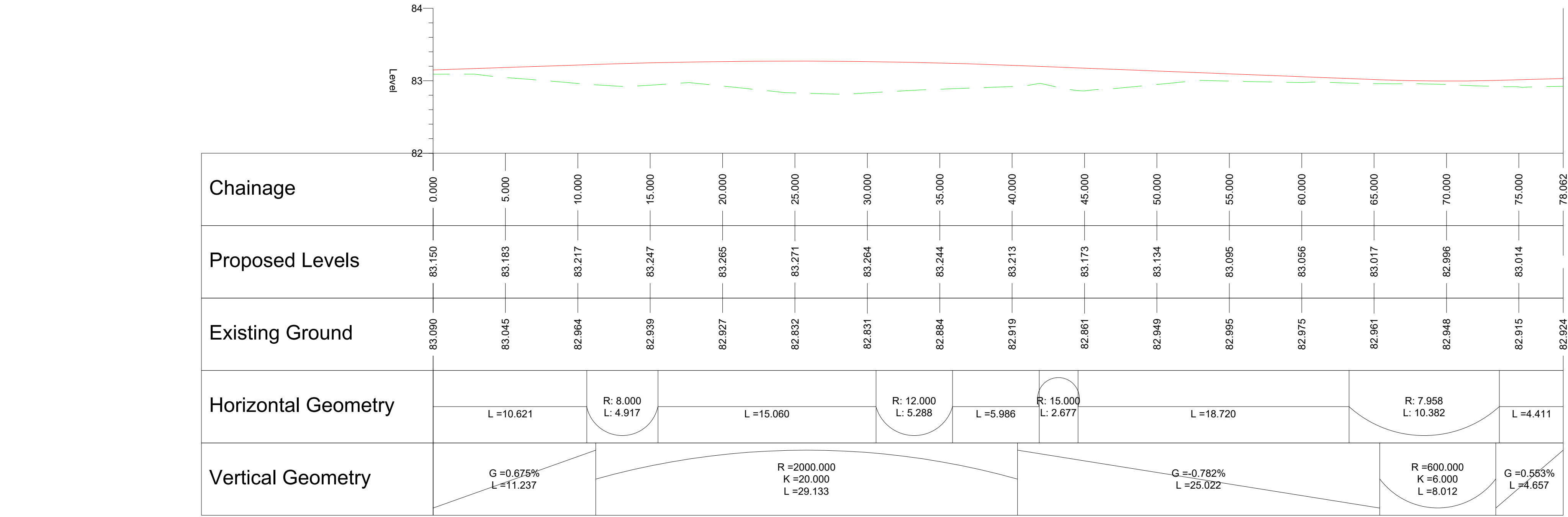
TURNING HEAD S KERB RETURN - LONGSECTION SCALE: H 1:200,V 1:40. DATUM: 82.000
