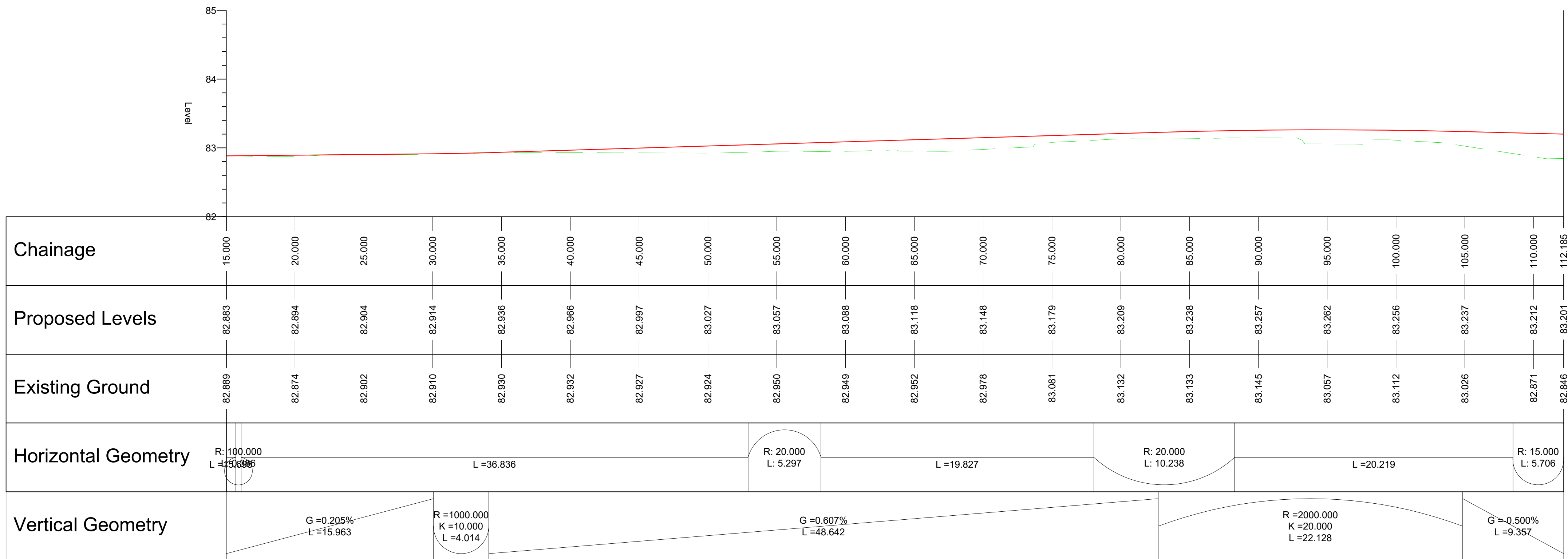
ALIGNMENT - ACCESS RD CL - LONGSECTION SCALE: H 1:200,V 1:40. DATUM: 82.000
