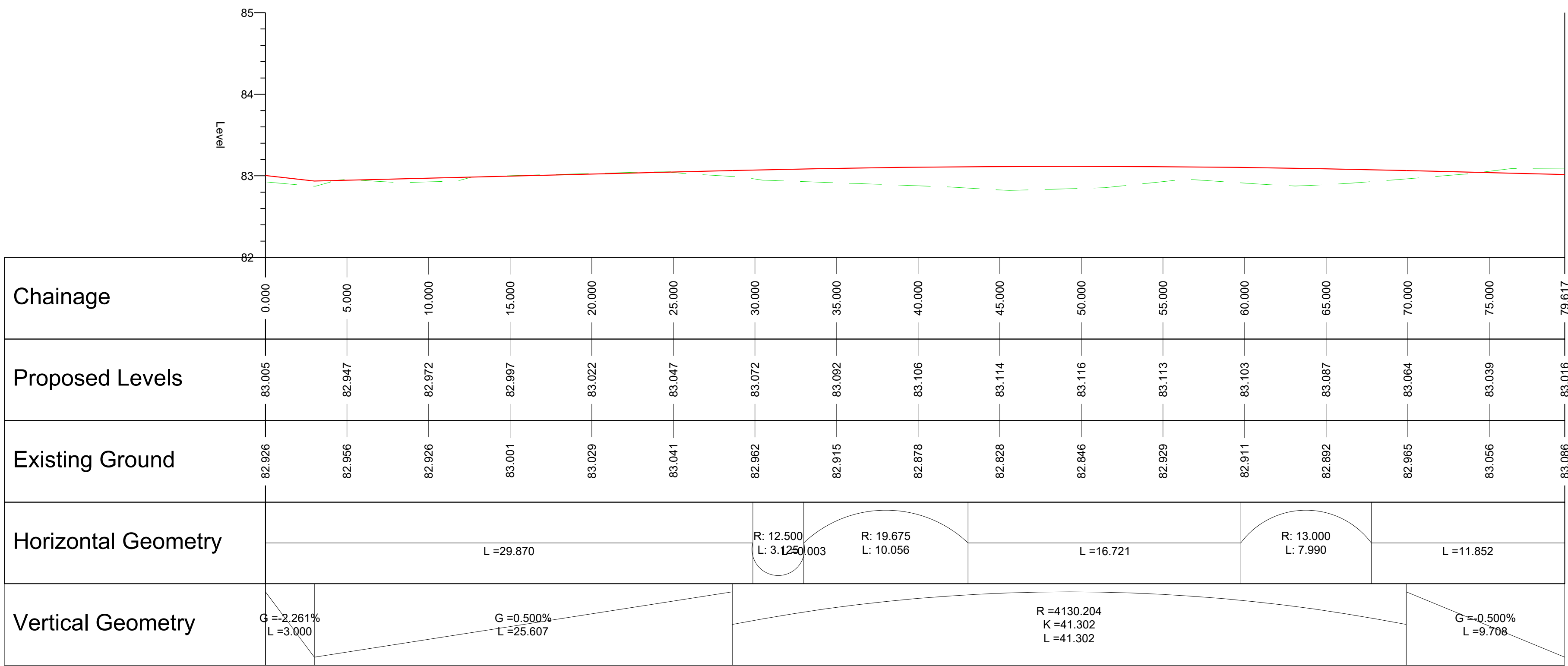
ALIGNMENT - TURNING HEAD CL - LONGSECTION SCALE: H 1:200,V 1:40. DATUM: 82.000
