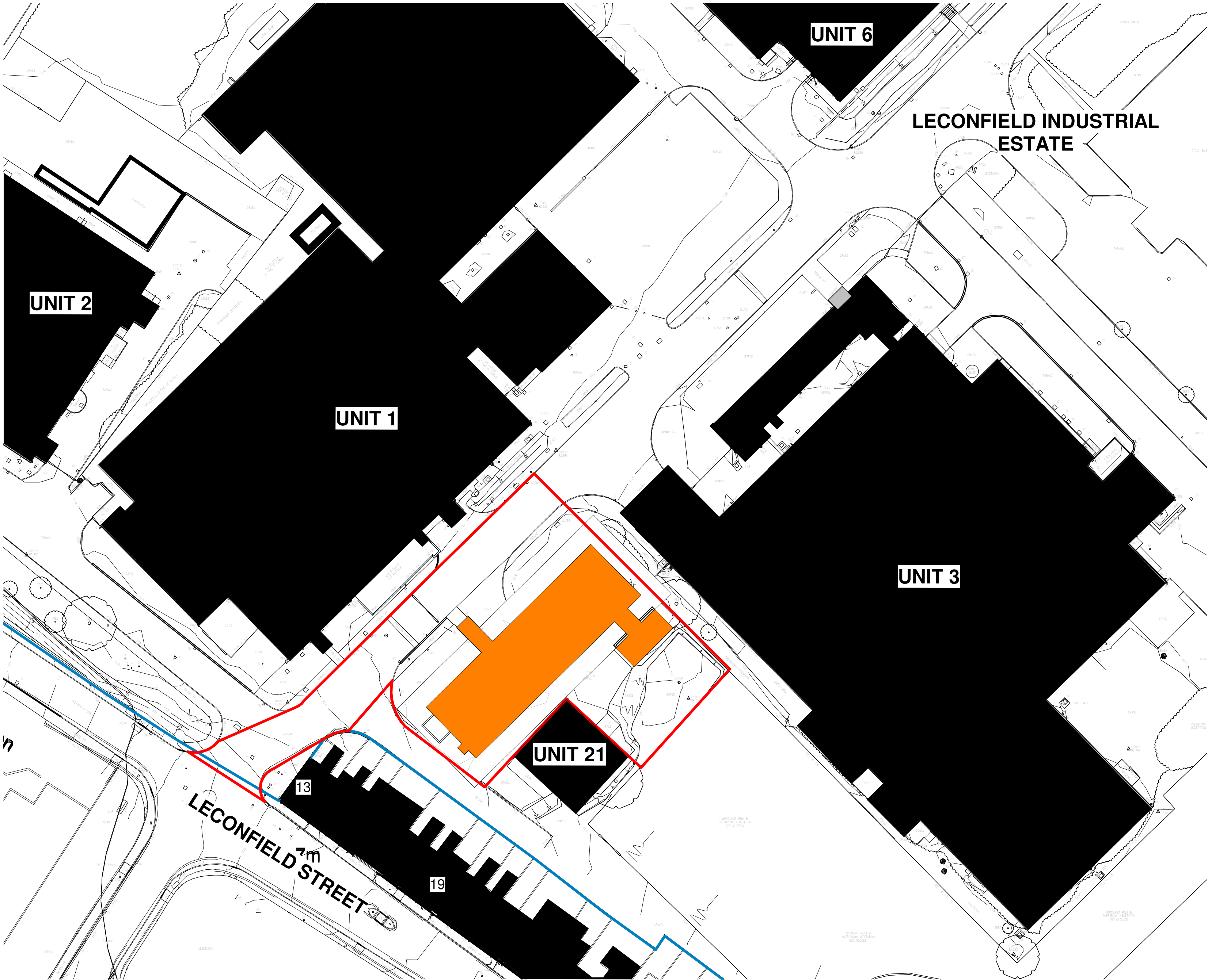
SITE - EXISTING BLOCK PLAN SCALE: 1 : 500
