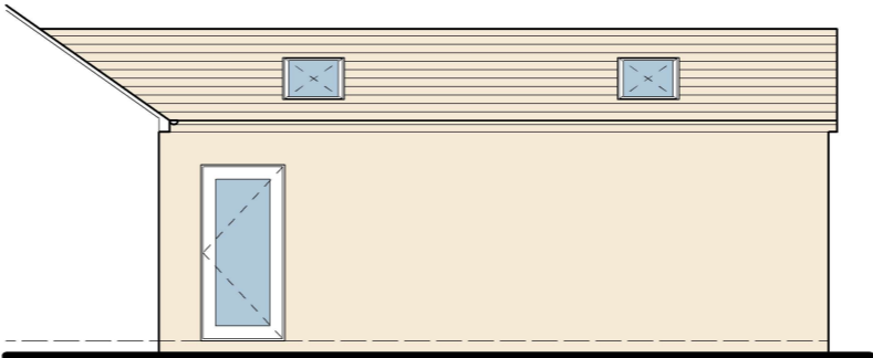
RIGHT HAND ELEVATION @ 1:100
