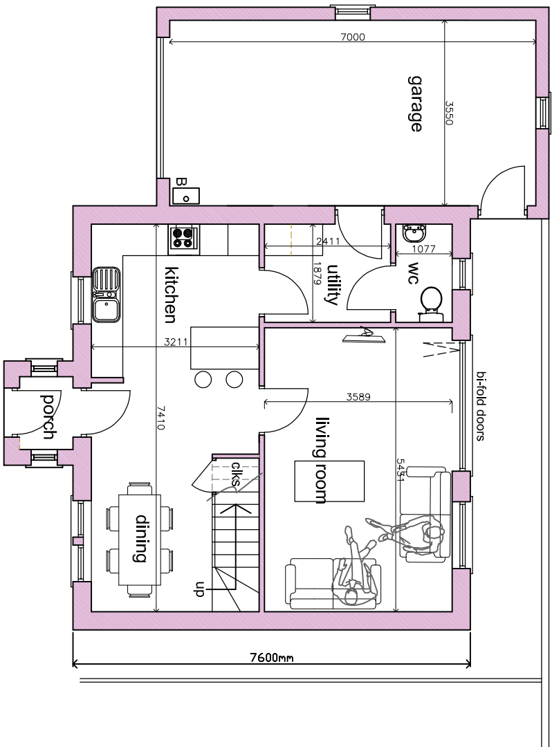
GROUND FLOOR PLAN 1:100 G/F = 52sq.m
