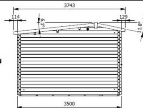
SIDE ELEVATION View D
