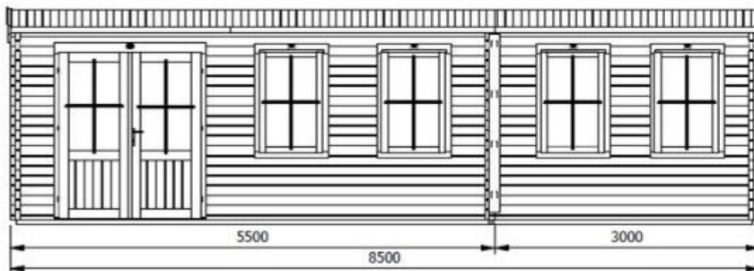
FRONT ELEVATION View A
