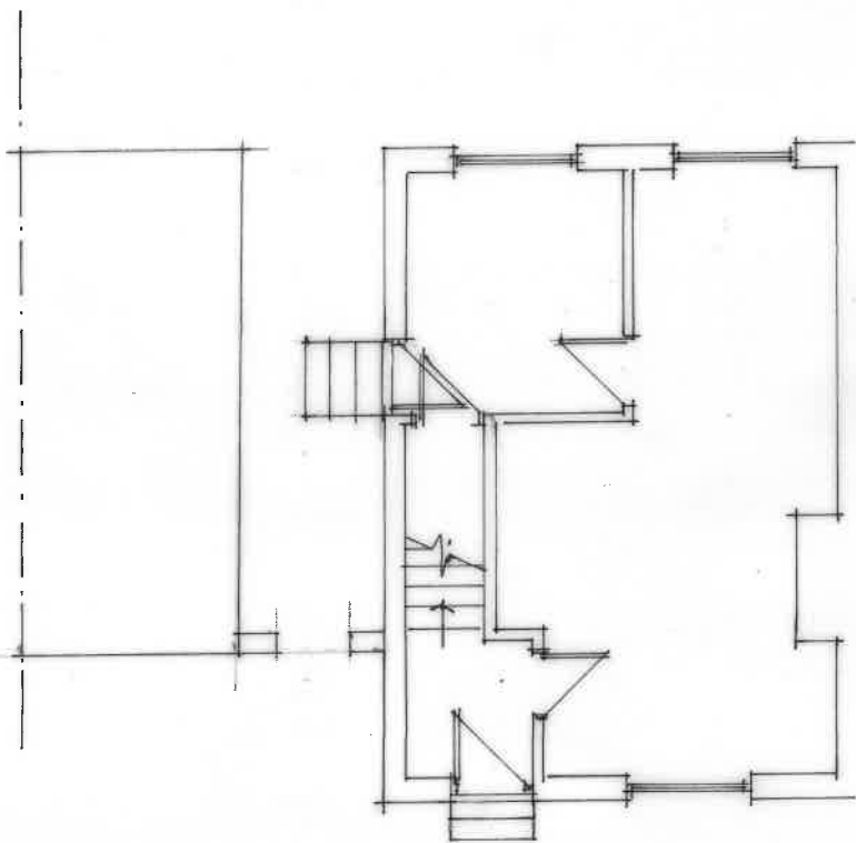
EXISTING GF PLAN
