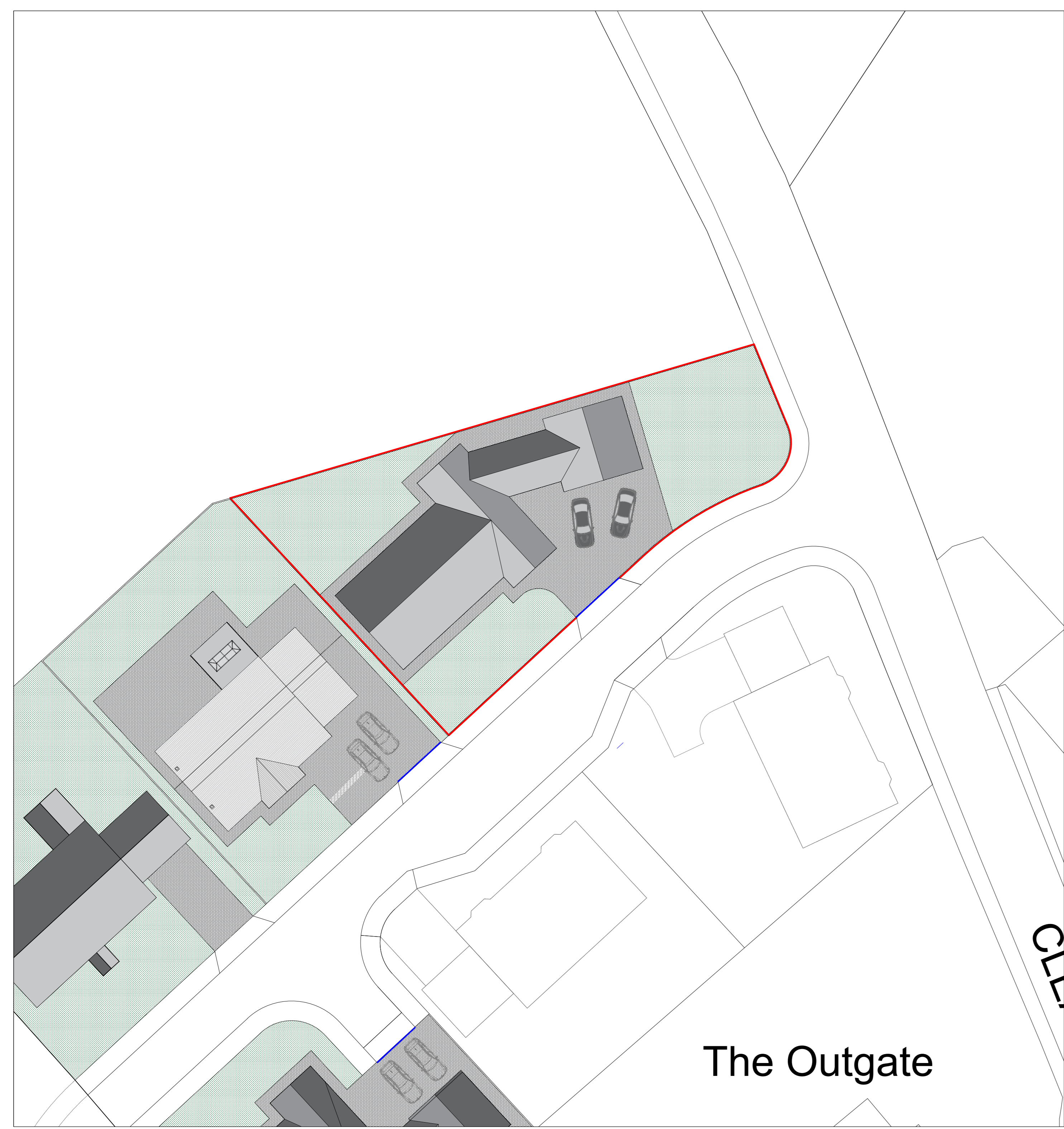
Proposed Block Plan 1/200
