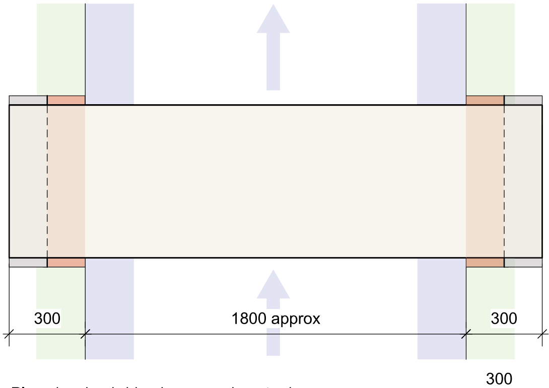
Plan showing bridge in comparison to river
