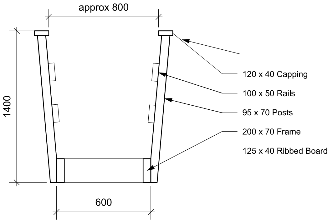
Front Elevation
