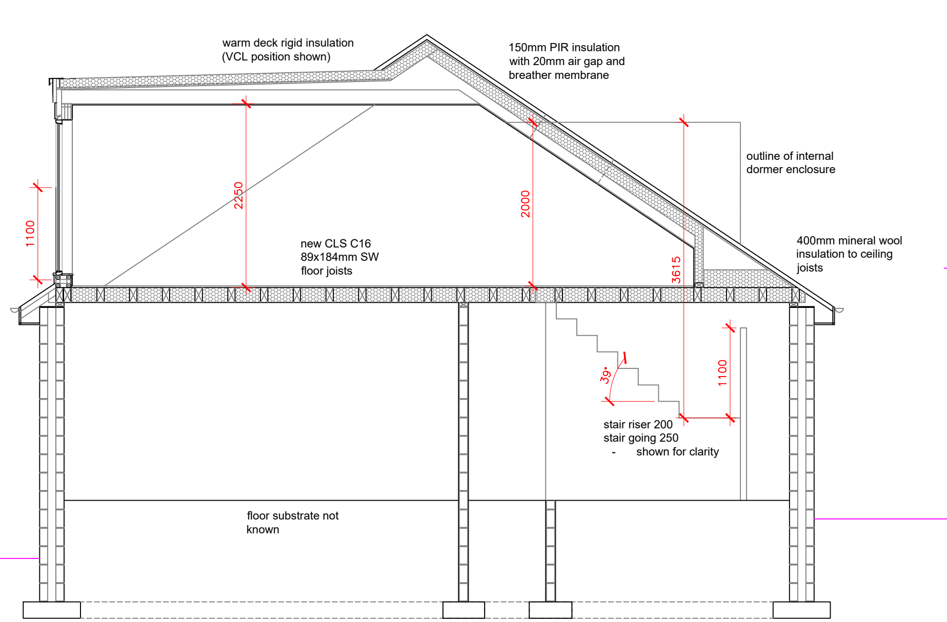
Section
