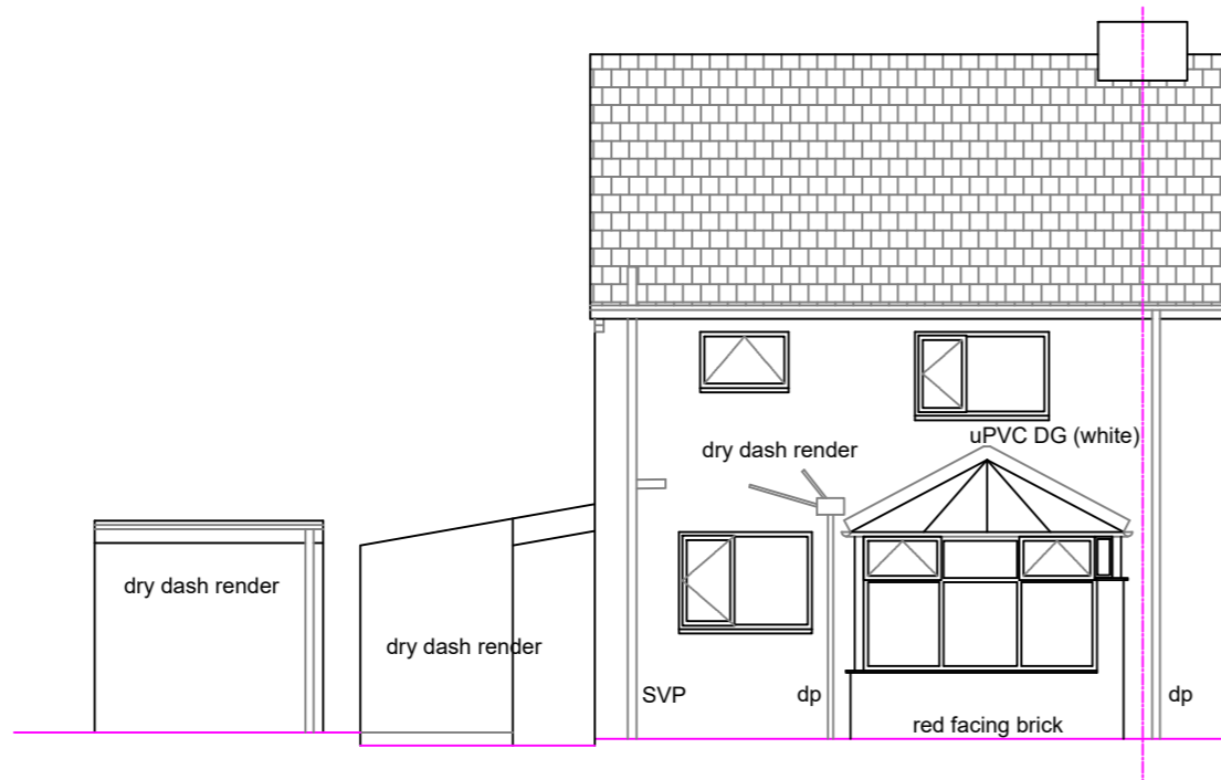
Rear Elevation
