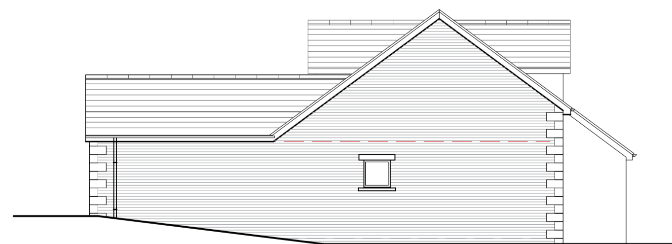
SIDE ELEVATION
