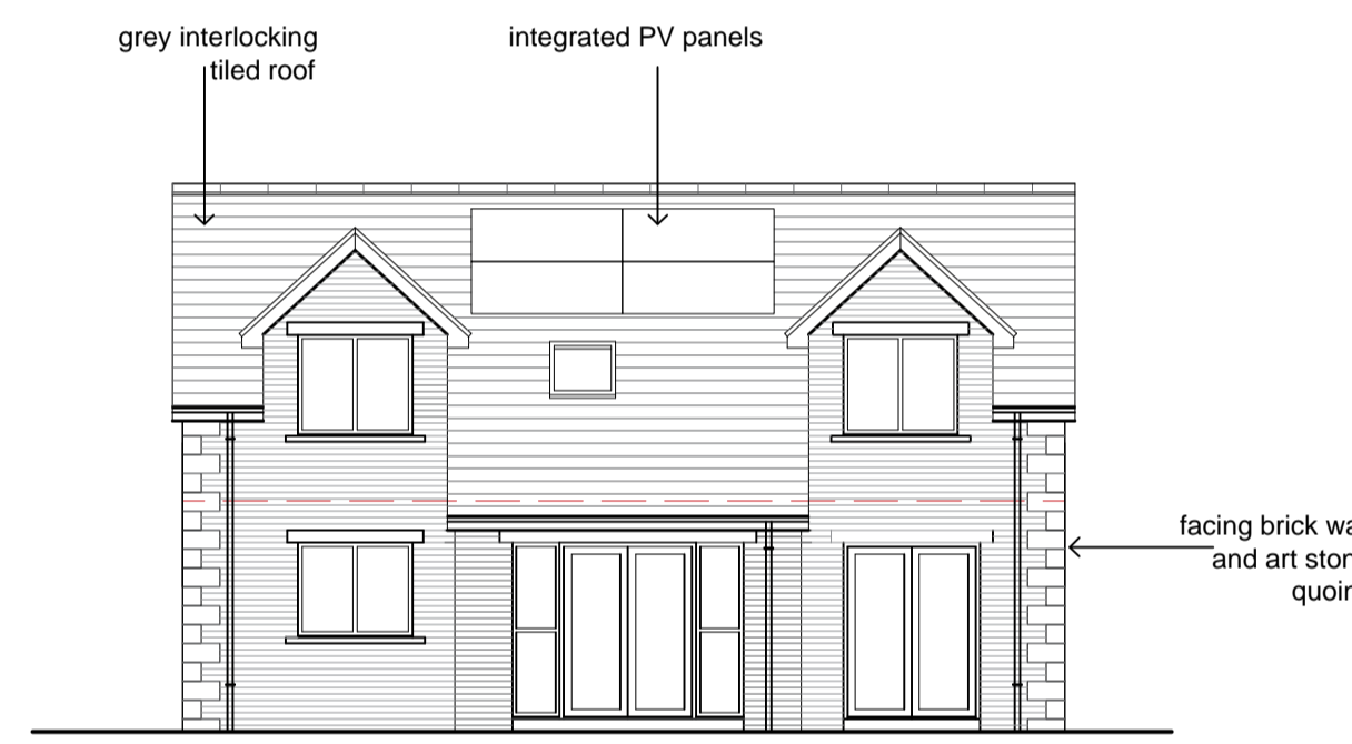
REAR ELEVATION
