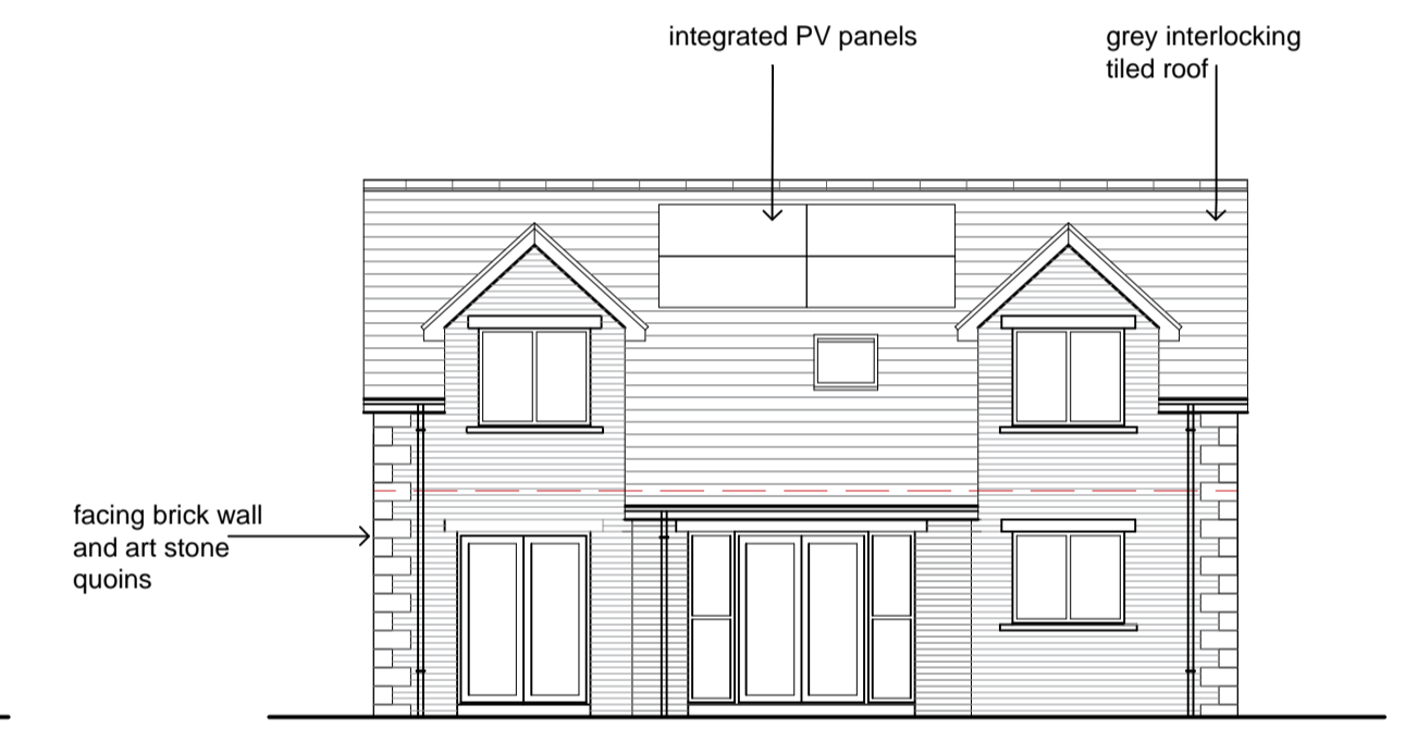
REAR ELEVATION
