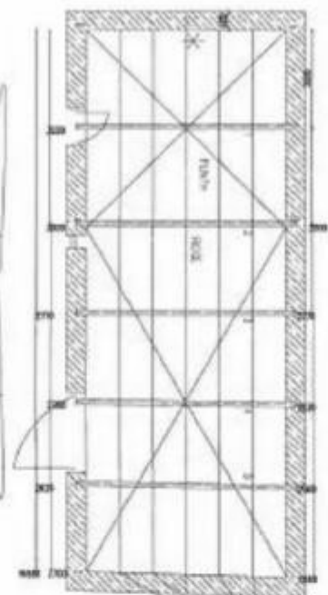
PLAN SHOWING ROOF TIMBER LAYOUT (EXISTING) FIRST FLOOR PLAN
