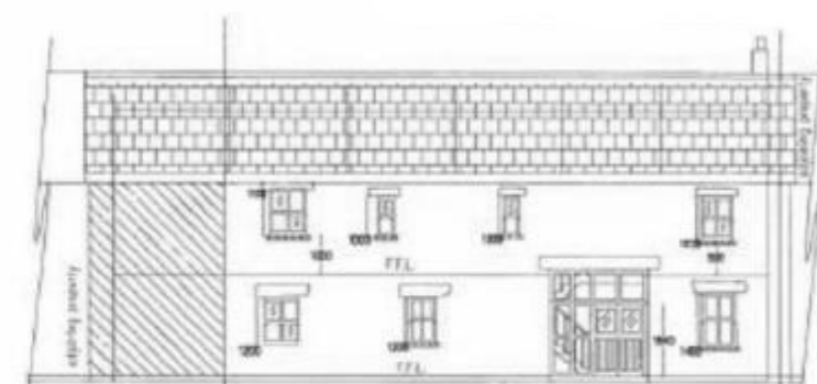
FRONT ELEVATION
