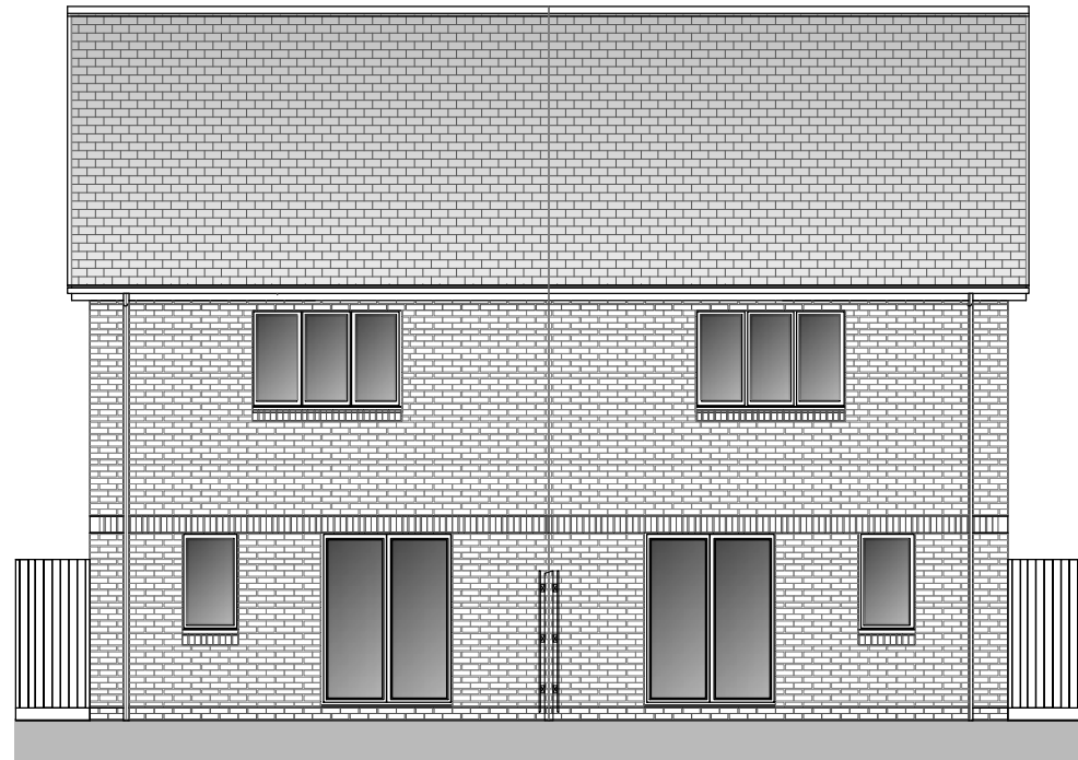
REAR ELEVATION
