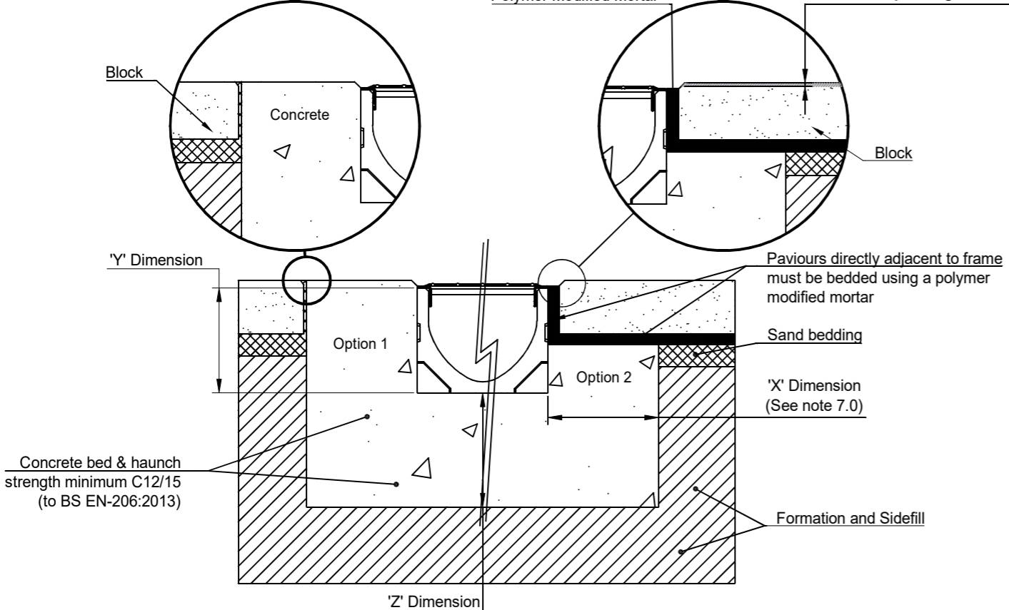
1 : 5 ACO RainDrain Block Pavement (Option 1 and 2)
