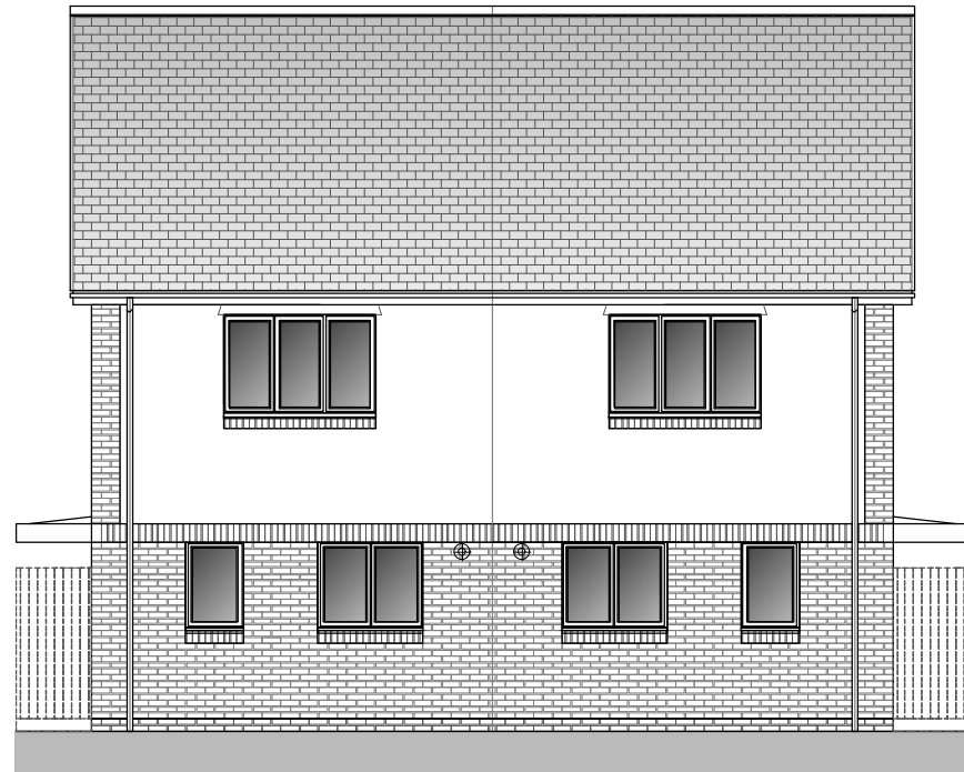
FRONT ELEVATION
