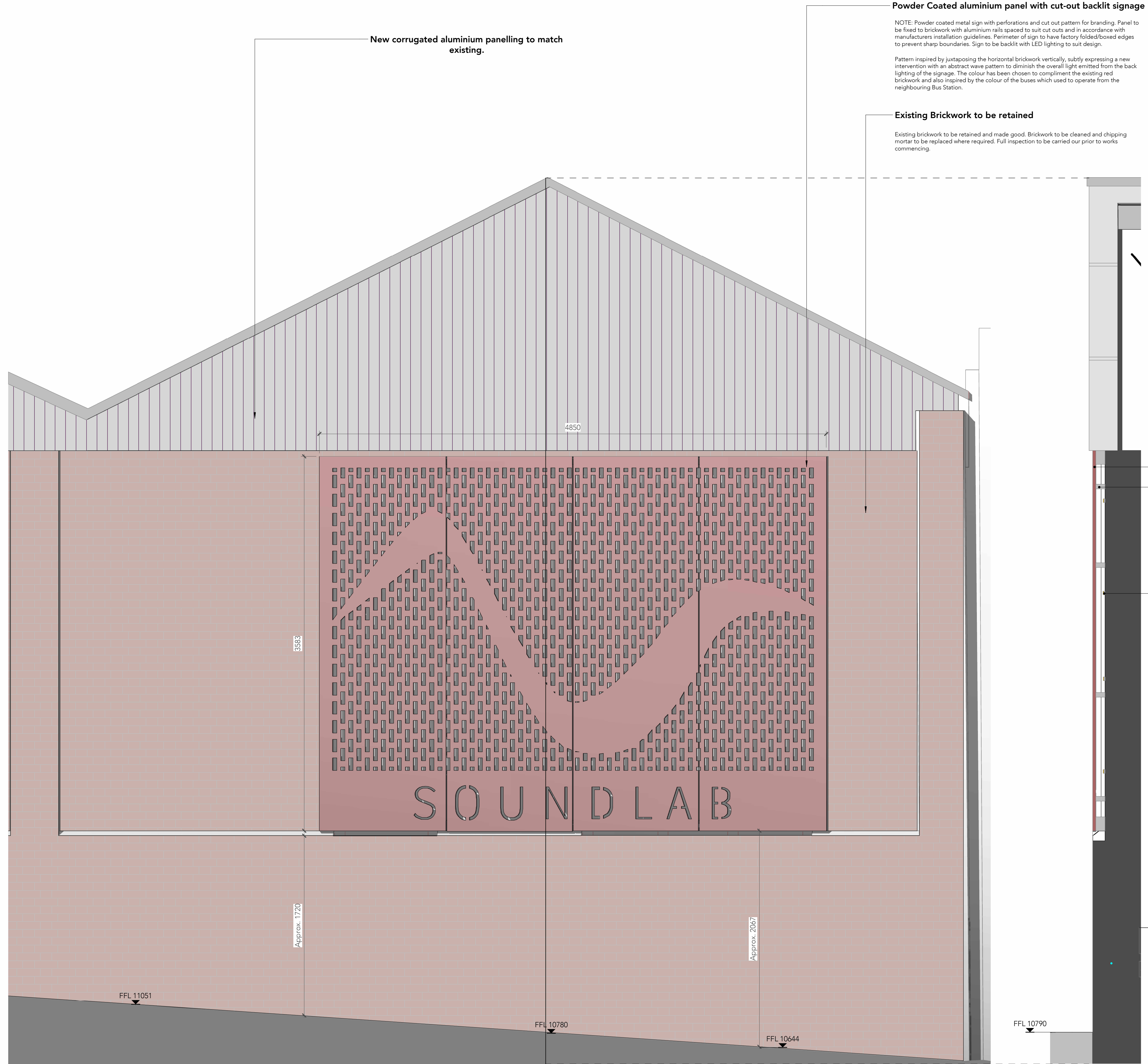
1 North Elevation - Signage Elevation 1 : 20
