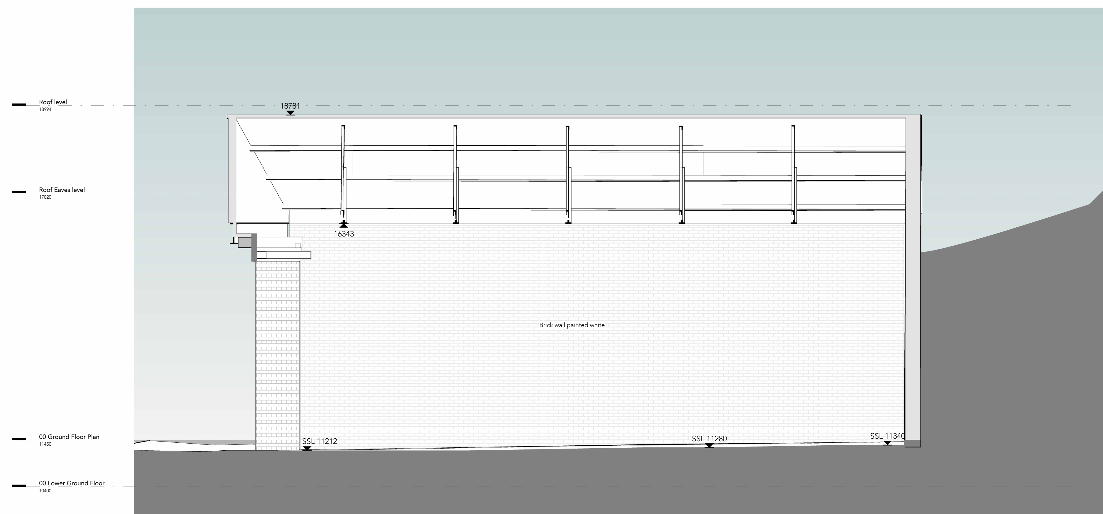
1 Section 1 1:50
