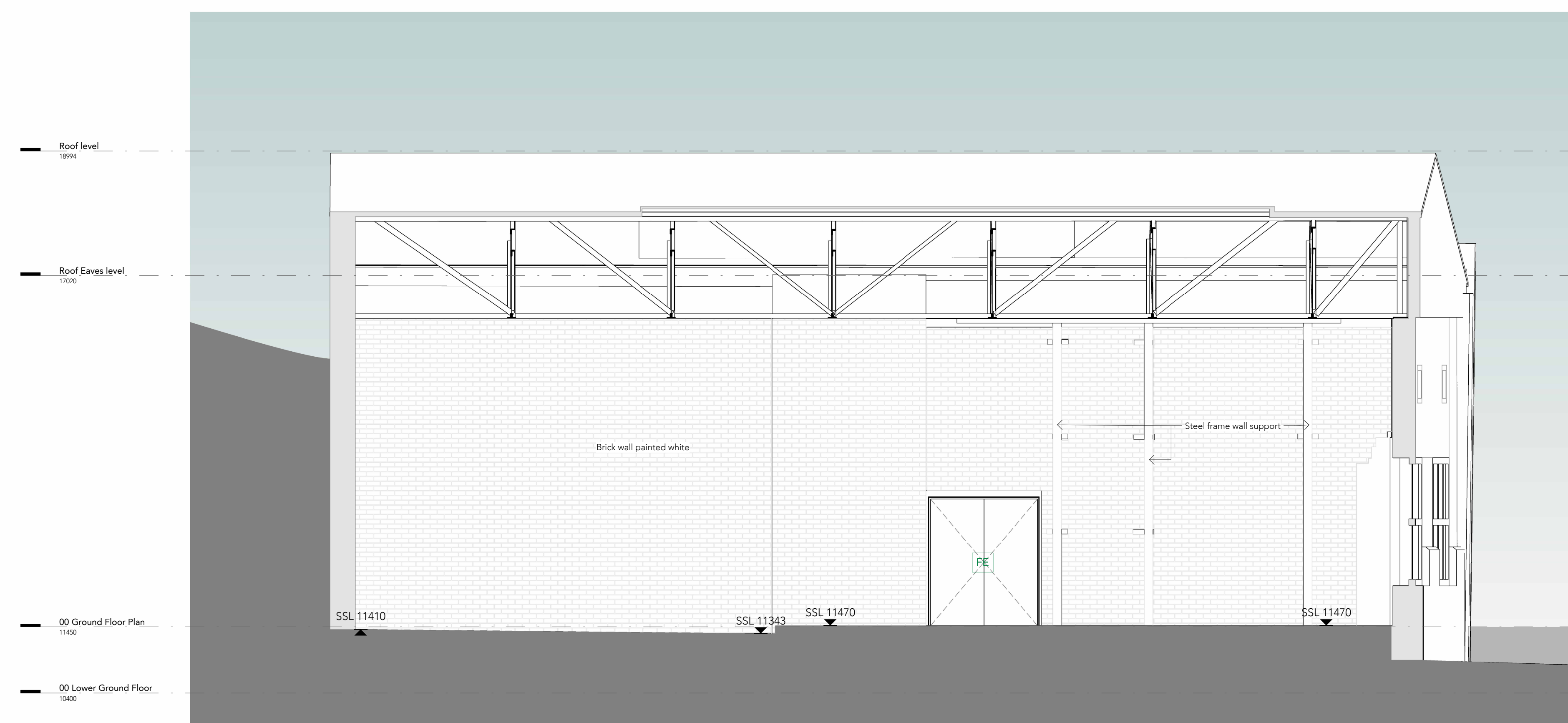
2 Section 2 1:50
