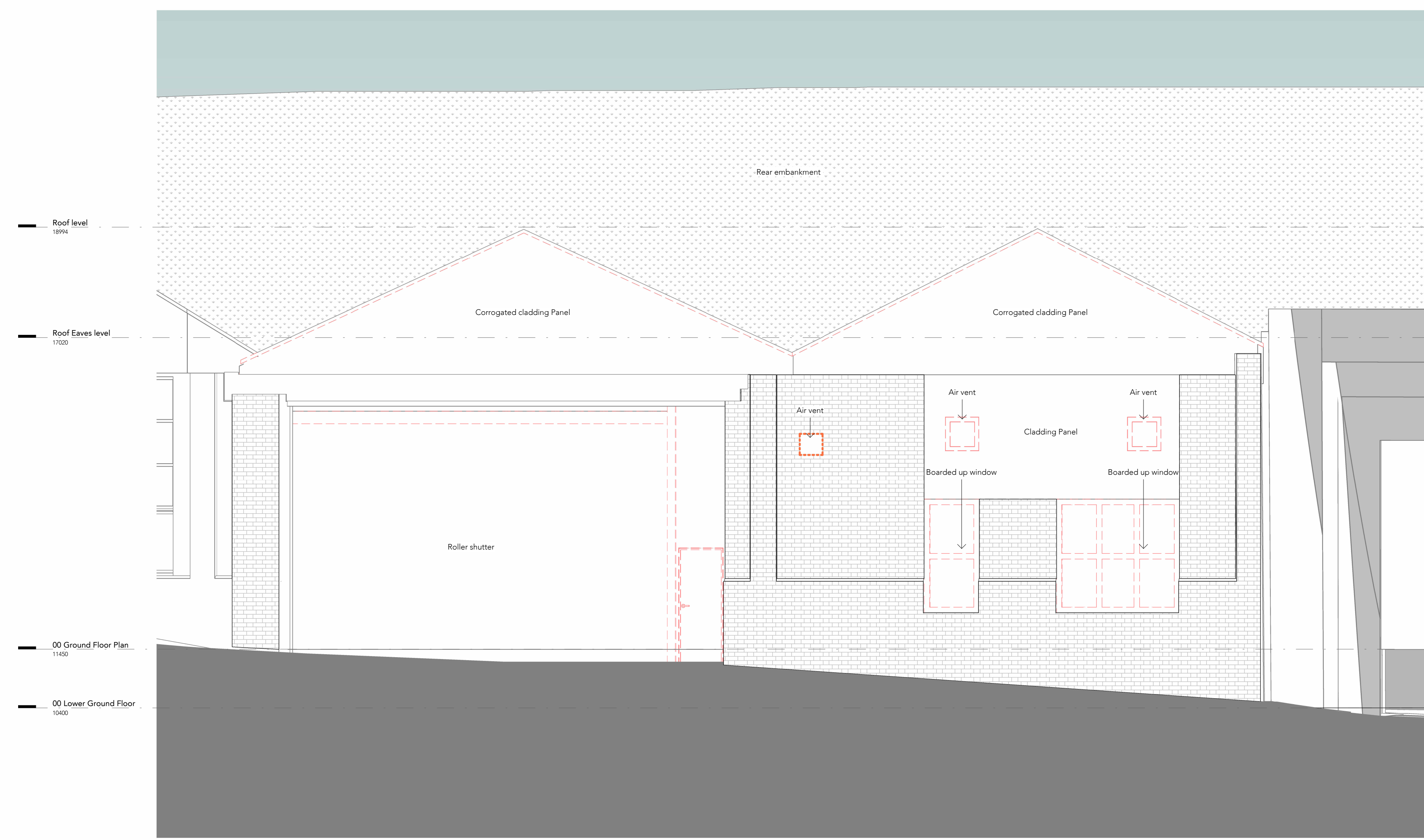
1 North Elevation - Demolition 1:50
