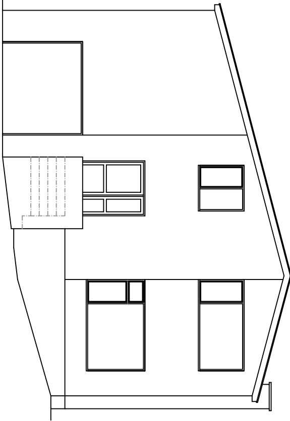
South Elevation
