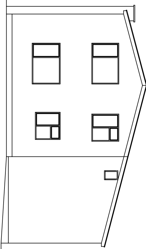
North Elevation
