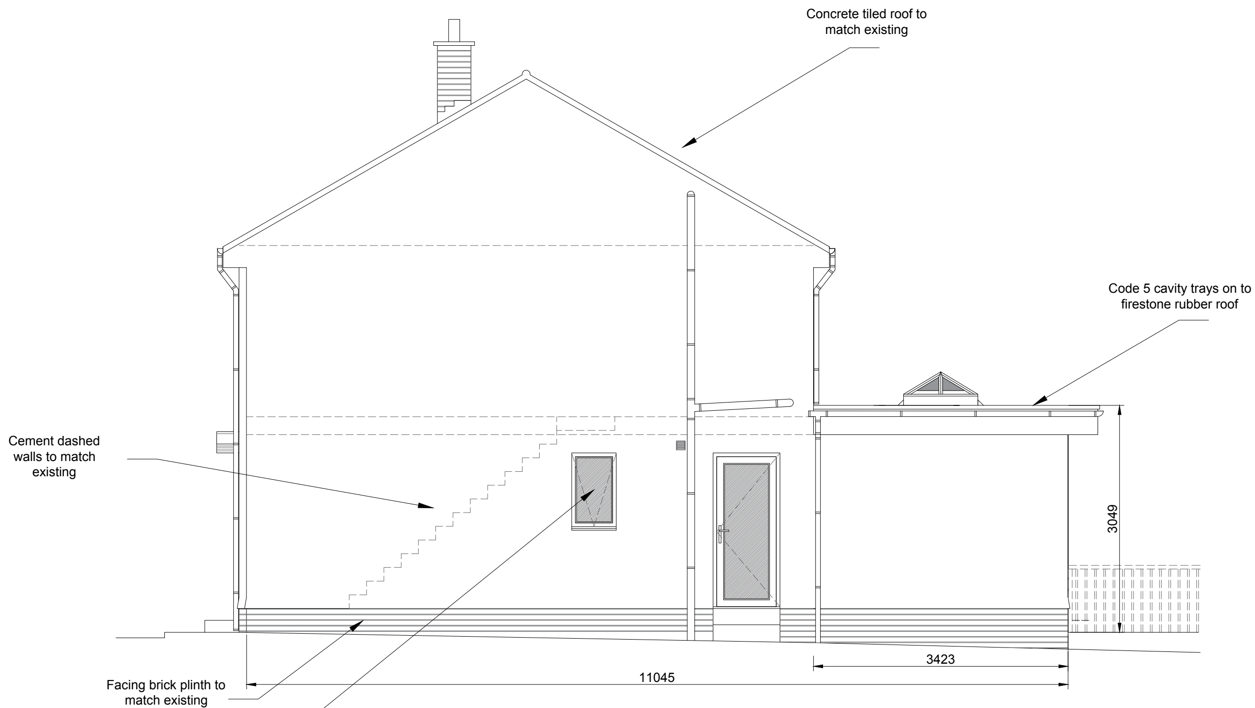
West Elevation
