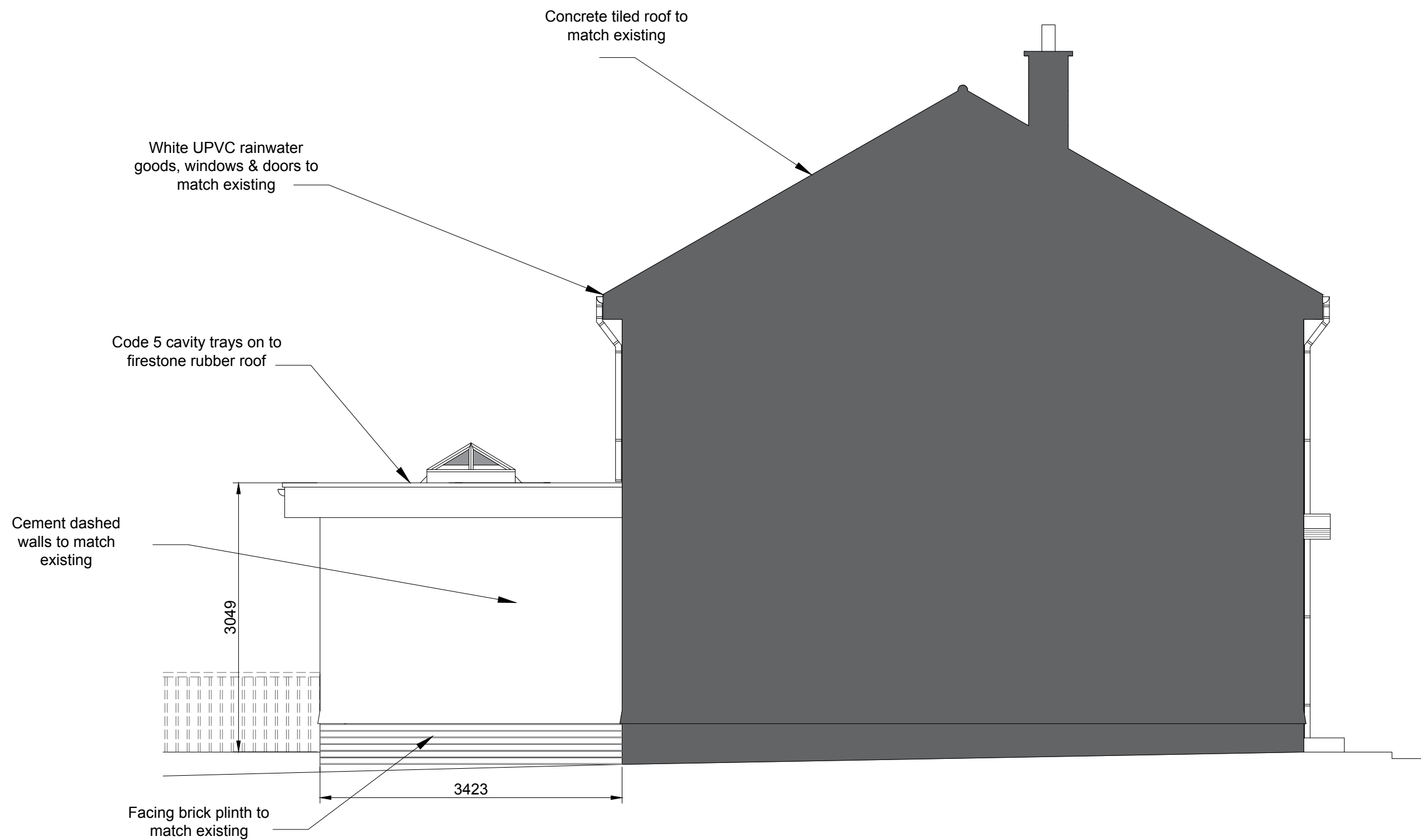
East Elevation
