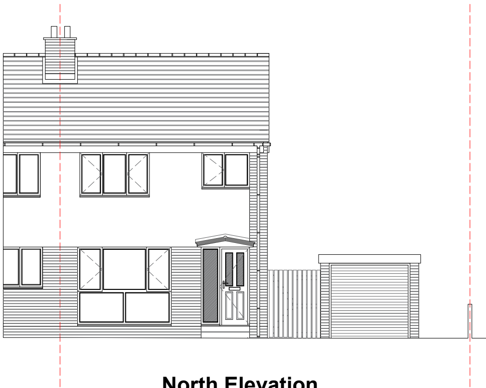
North Elevation
