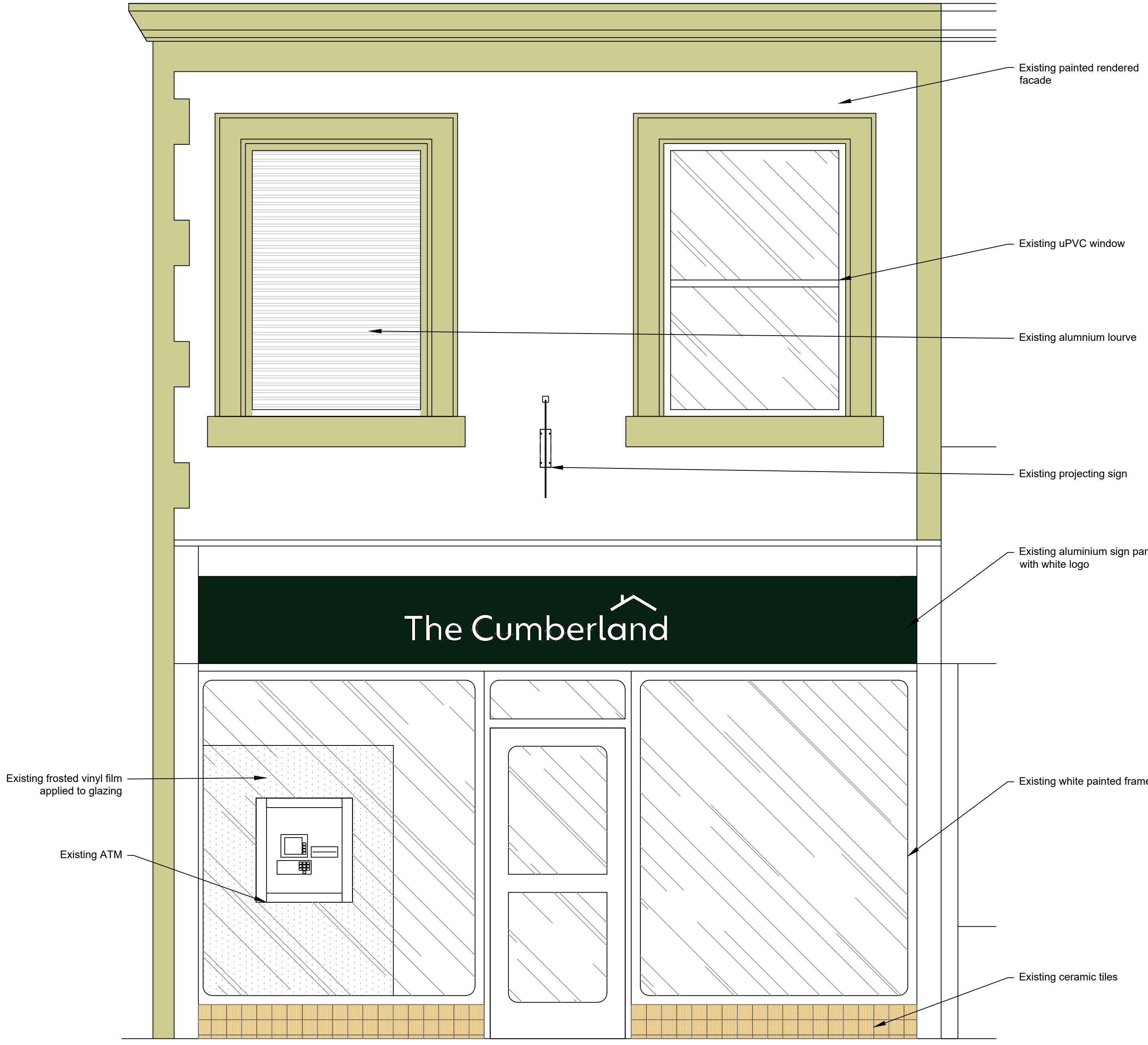
1 Existing Main Street Elevation Scale: 1:25@A1
