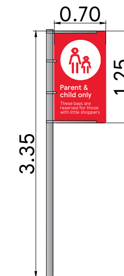
SIGN 14 0.70x3.35 m New Pole mounted Parent & Child sign
