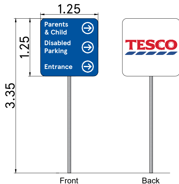
SIGN 11 & 12 0.70x3.35 m New Pole mounted Directional parking sign
