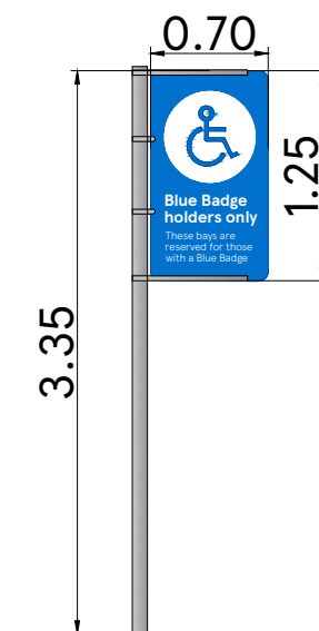
SIGN 13 0.70x3.35 m New Pole mounted Disable parking sign
