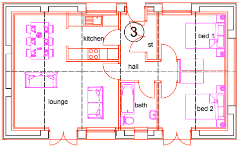
Proposed Ground Floor Plan - 68m2
