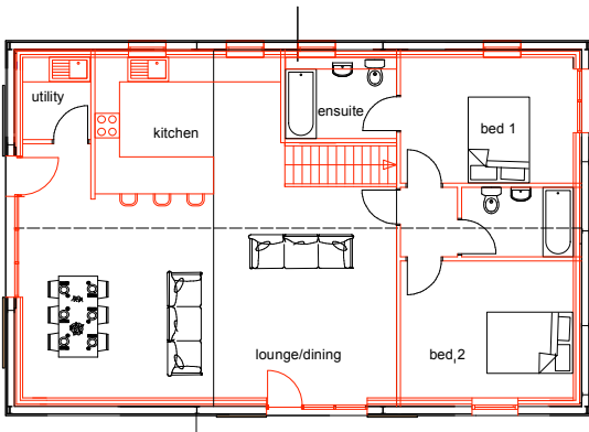
Proposed Ground Floor Plan - 112m2
