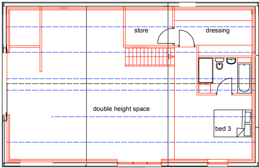
Proposed First Floor Plan - 36.5m2
