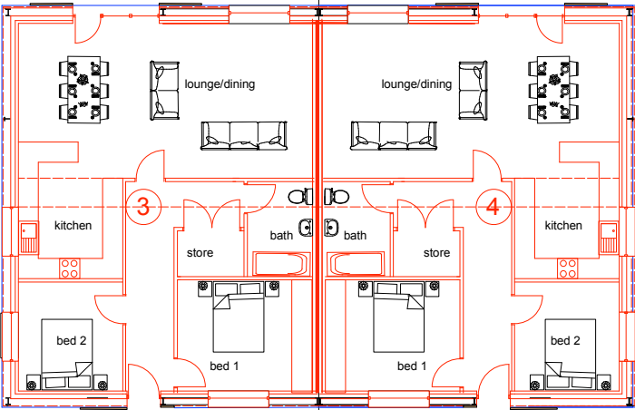
Proposed Ground Floor Plan - 95.5m2
