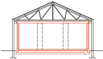
Proposed Section
