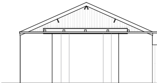
Existing East Elevation
