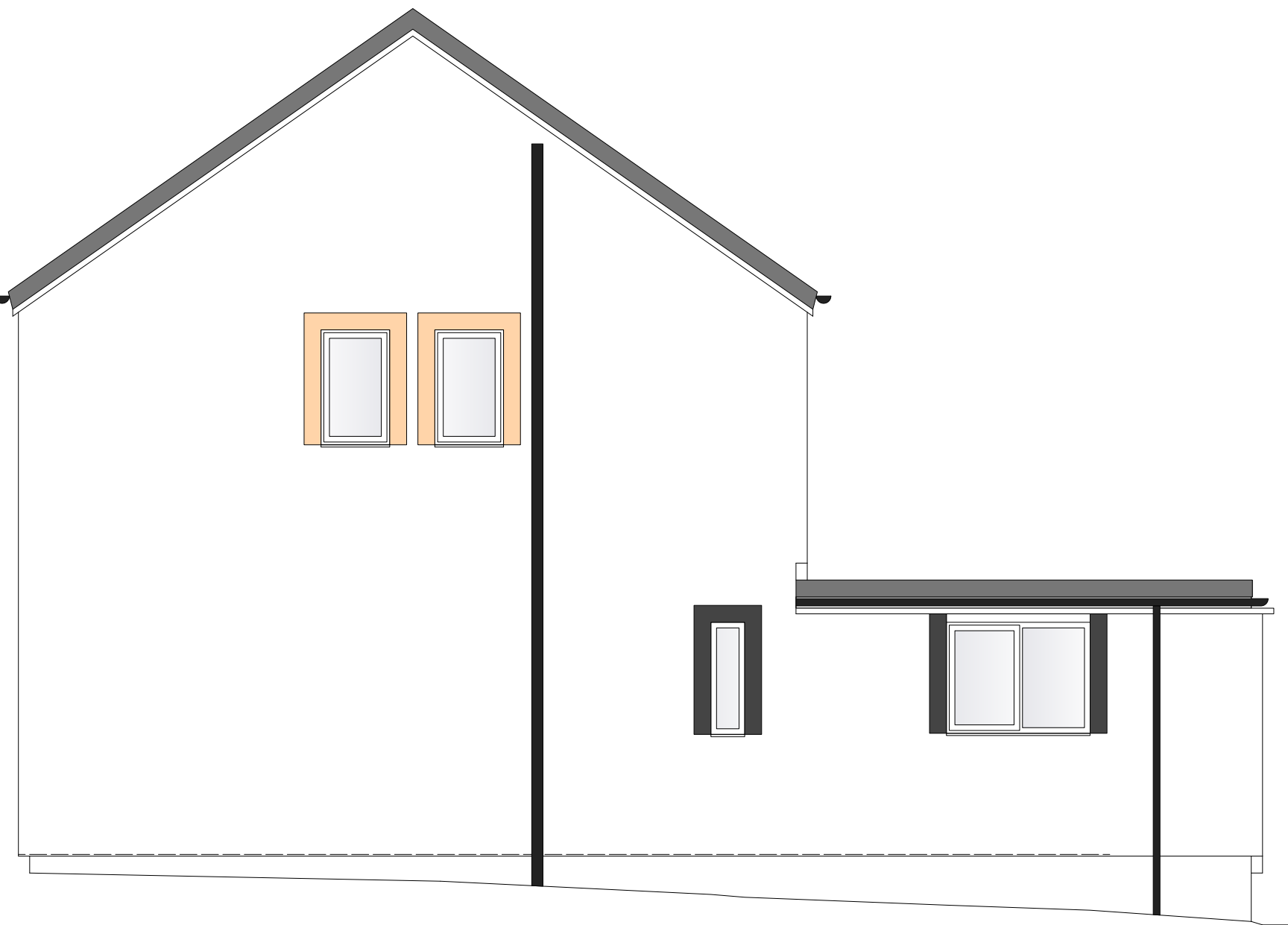
Side (East) Elevation As Existing Scale 1:50
