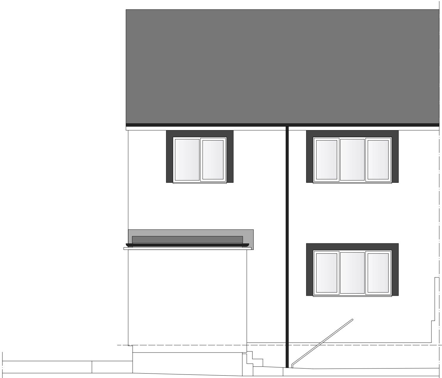
Rear (North) Elevation As Existing Scale 1:50
