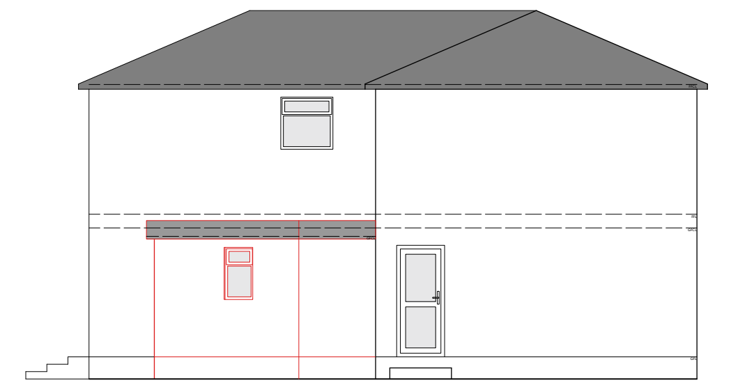
Side (North) Elevation As Proposed Scale 1:100
