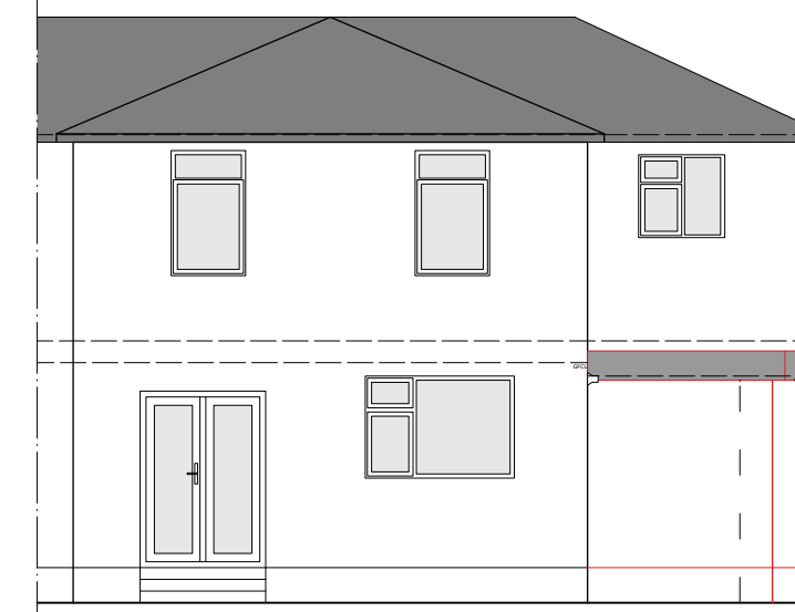
Rear (East) Elevation As Proposed Scale 1:100
