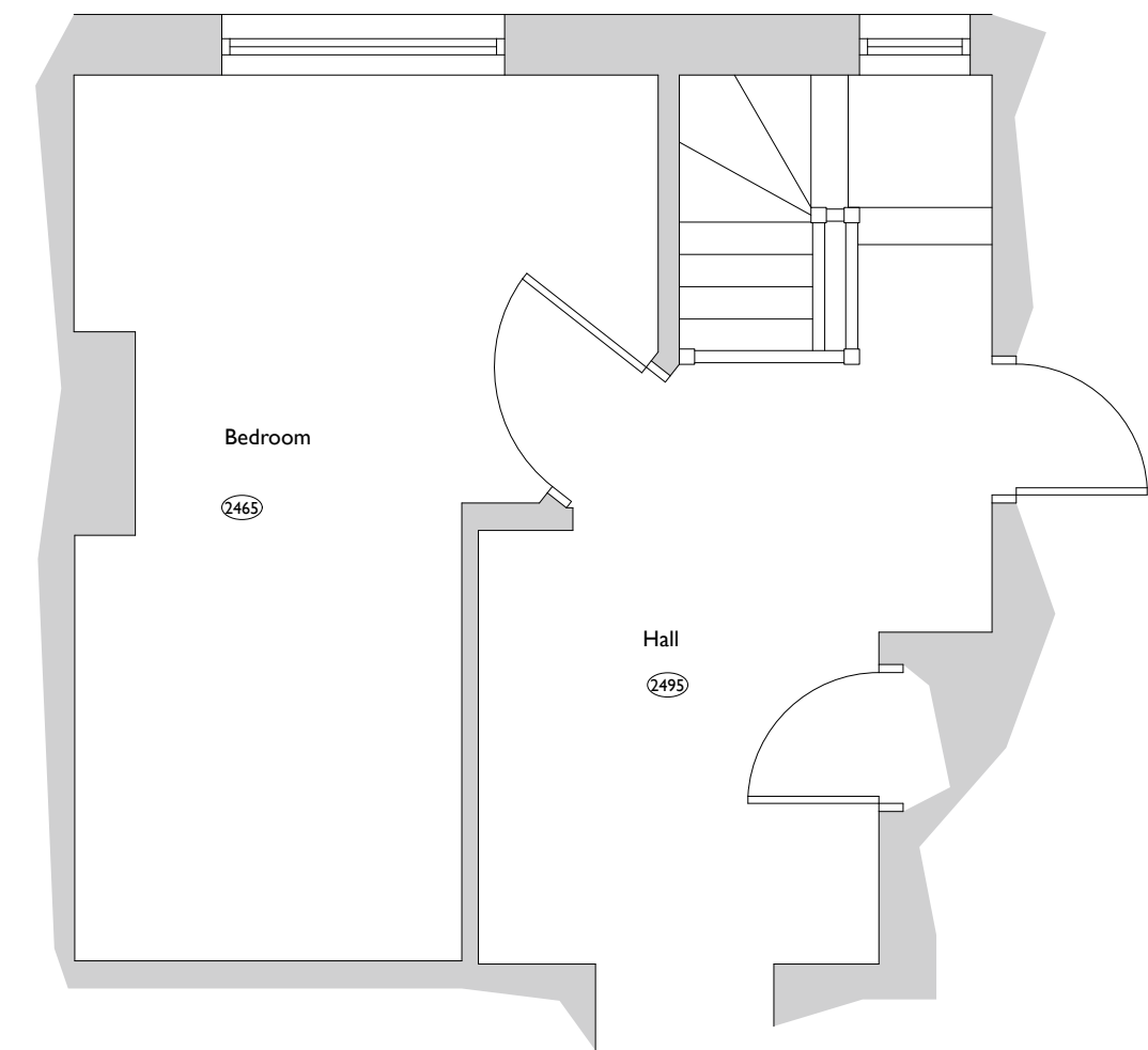
First Floor As Existing Scale 1:50
