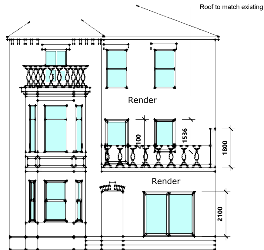
Existng Rear Elevation
