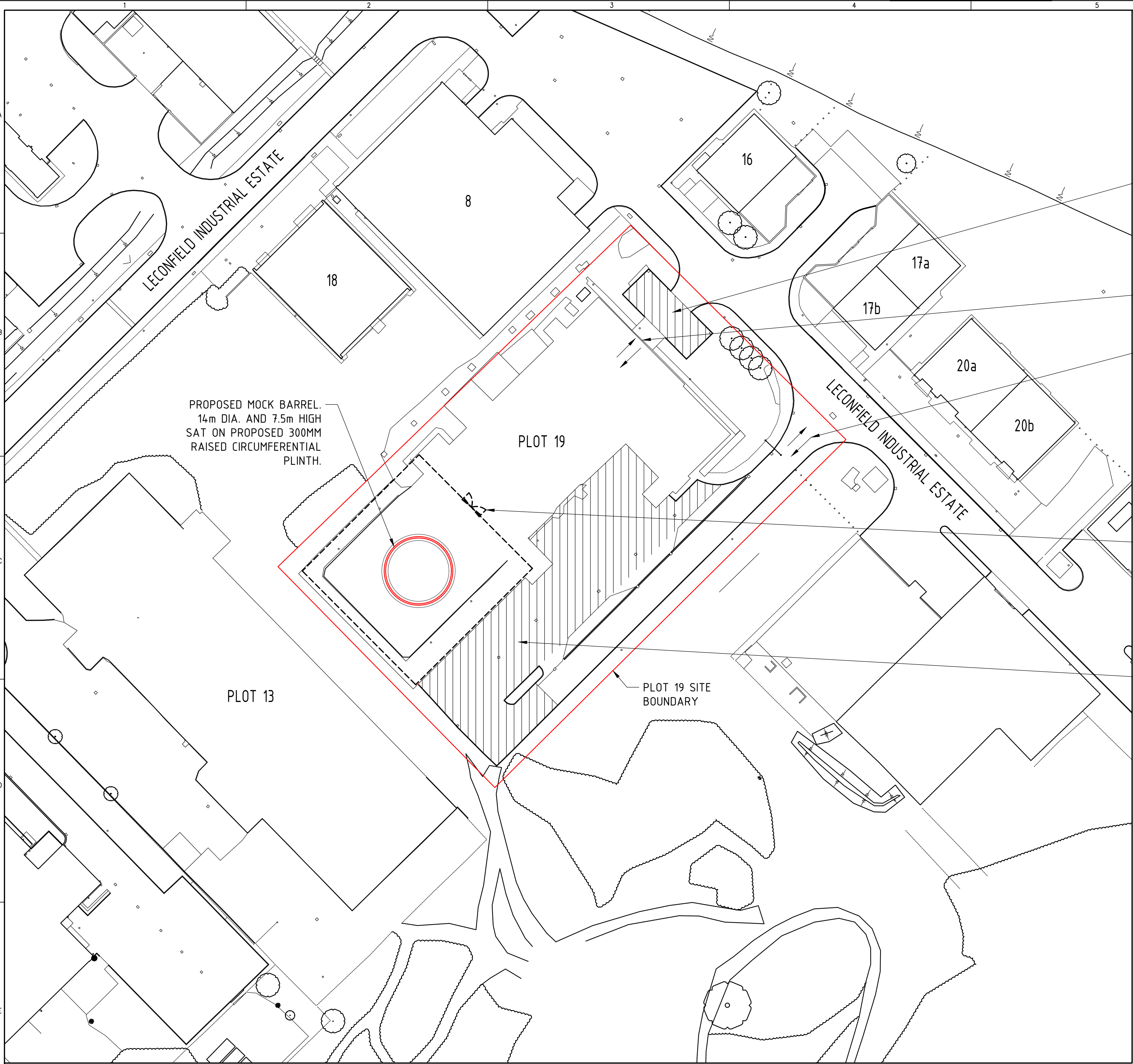
SITE / BLOCK PLAN SCALE 1:500
