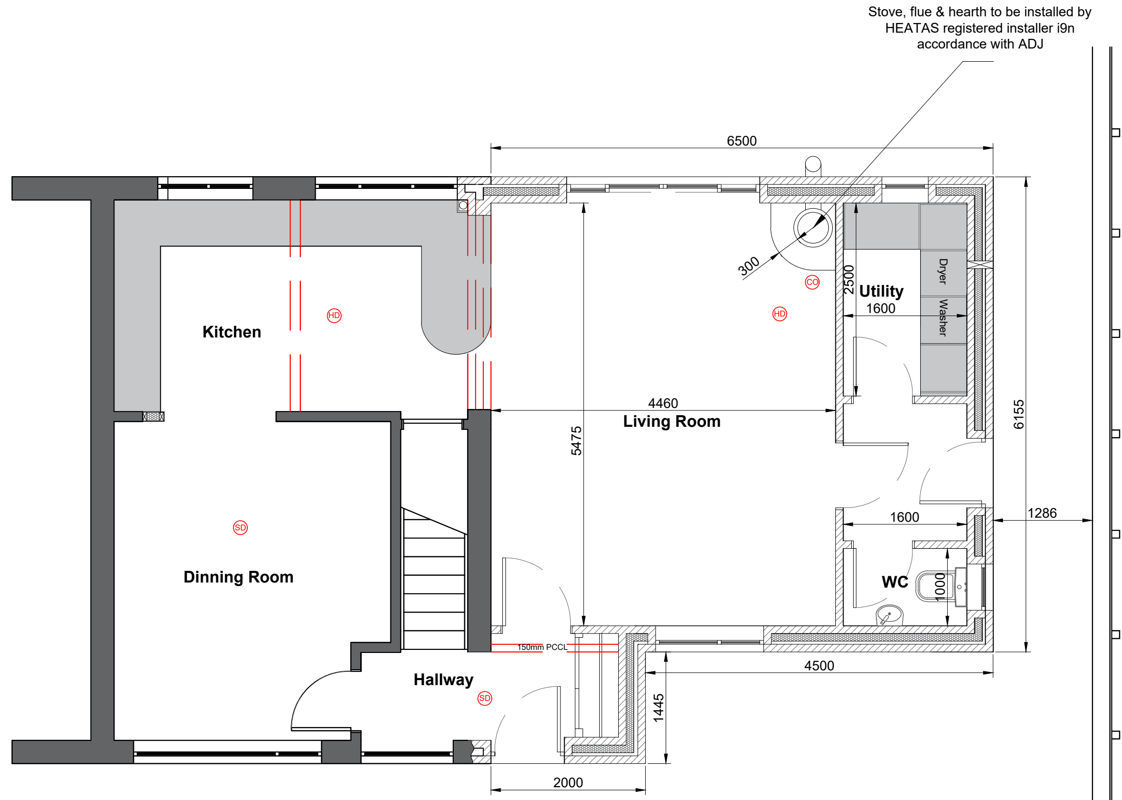
Proposed Ground Floor Plans
