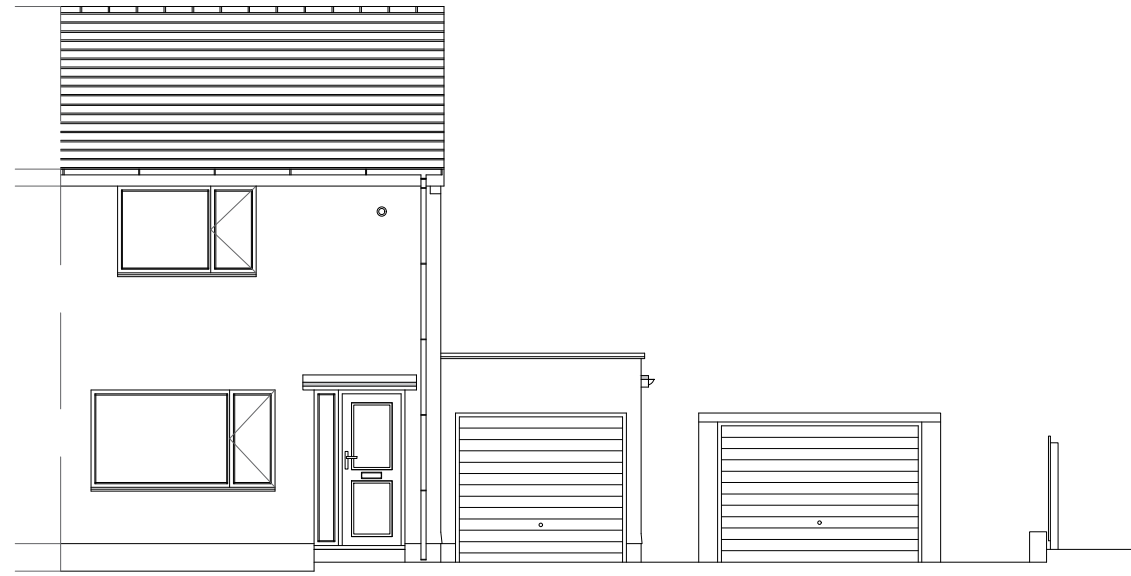
East Elevation
