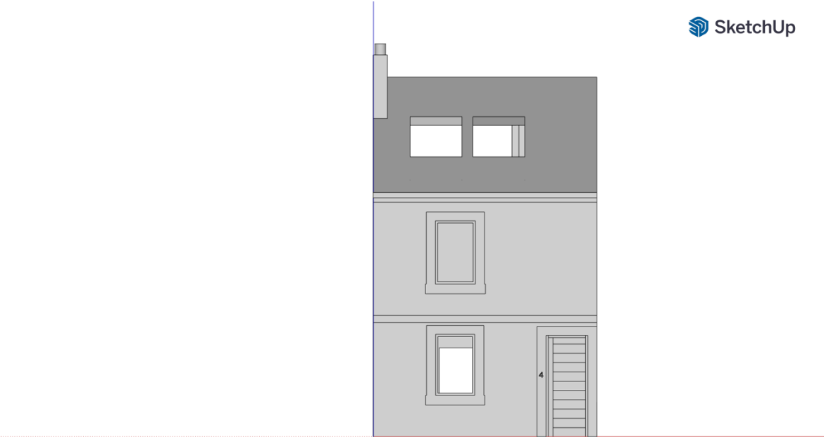
Figure 9: Front Proposed
