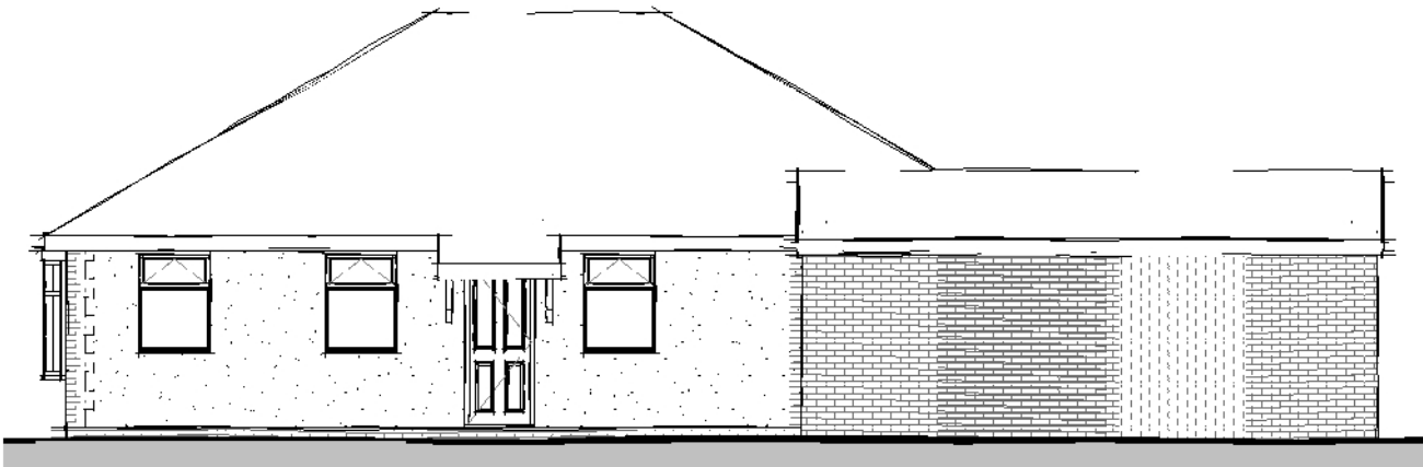
Side Elevation 01
