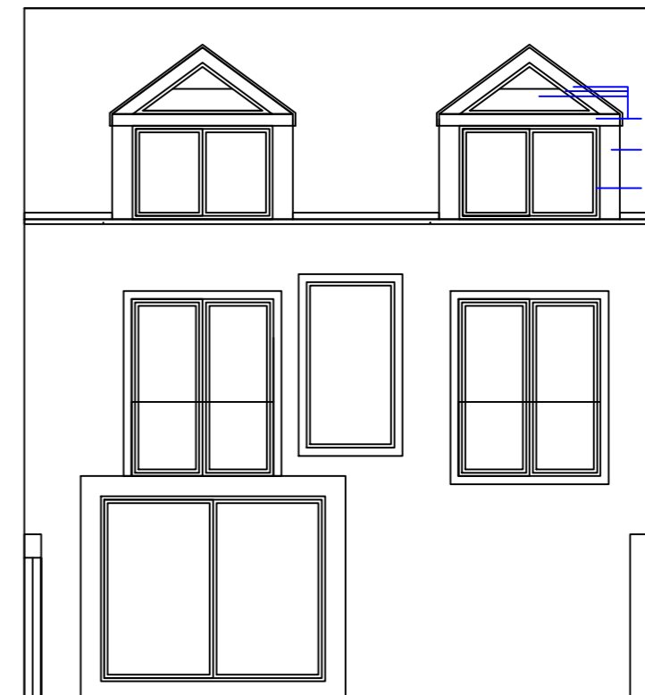
Rear Elevation
