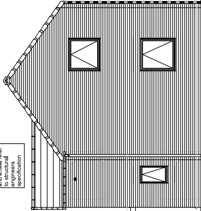
SIDE ELEVATION
