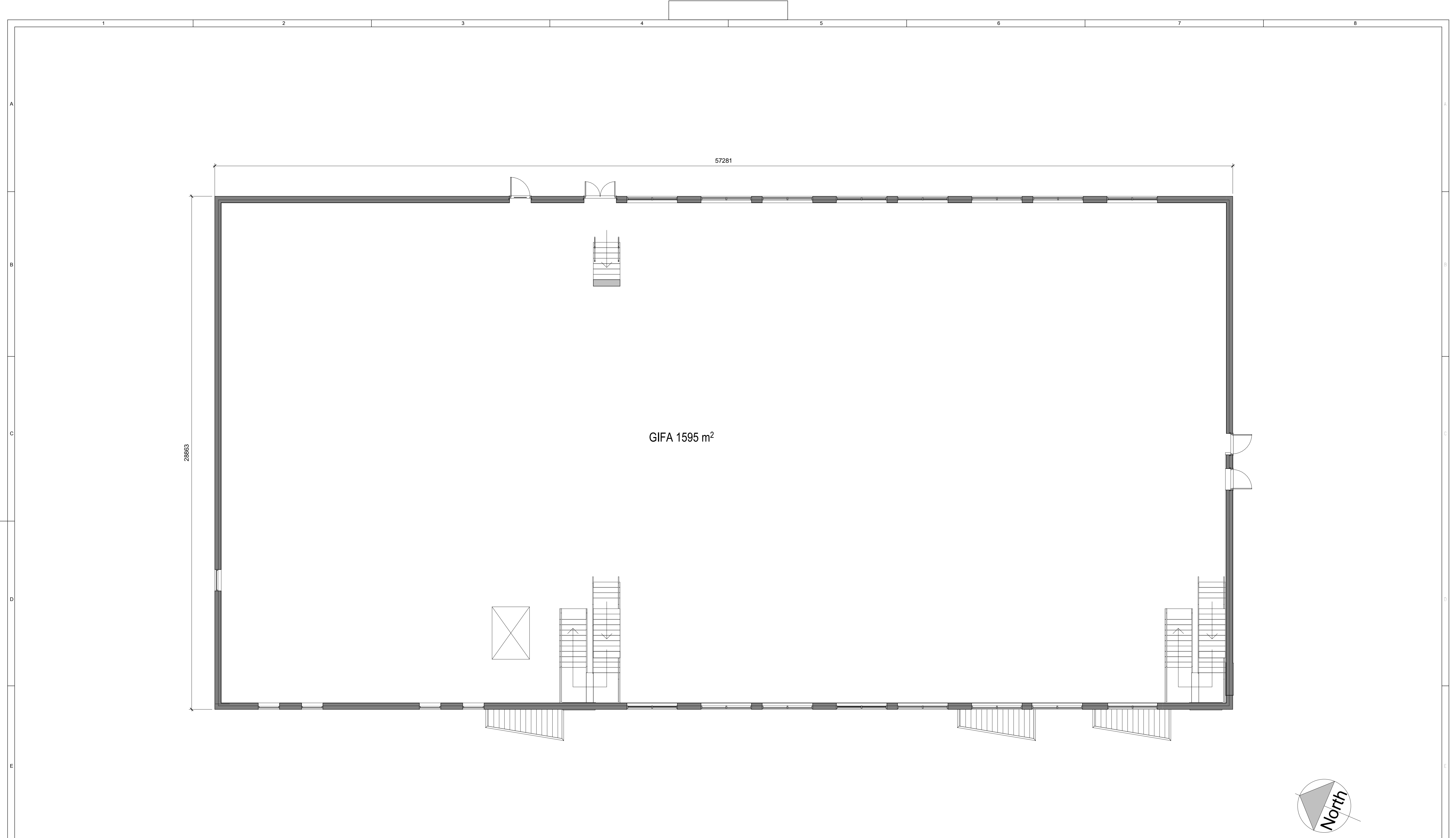
Proposed -0.000m Level Ground Floor Plan (40.28m AOD) 1 : 100
